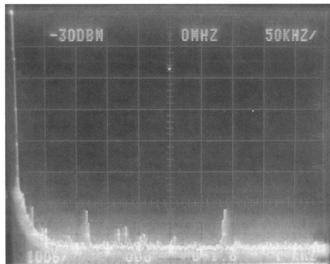
Figure 4. Spectrum analysis of RF signals present 100 m away from one high-voltage line.
