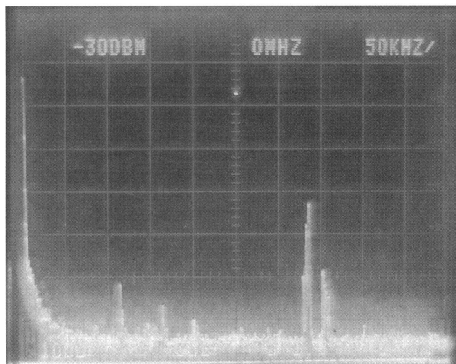
Figure 3. Spectrum analysis of RF signals present just under one high-voltage line.
